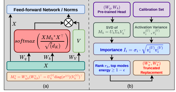
Figure 1: Conceptual representation of our proposed SVD-Attention is shown in (a). The SVD-Attention method is outlined in (b).
